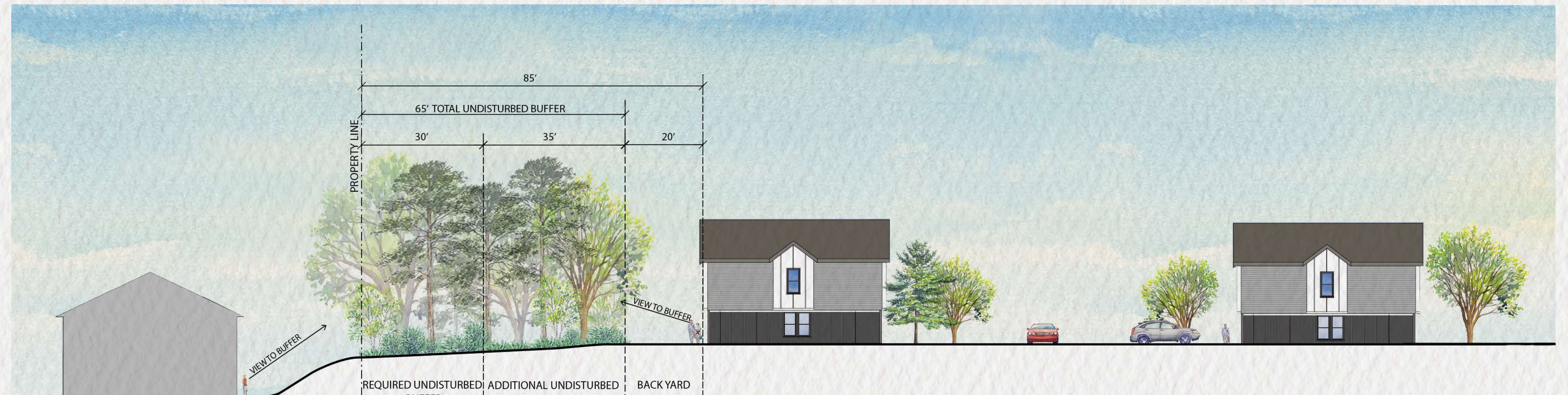
2 2-2 SECTION scale: 1"=16'-0"
