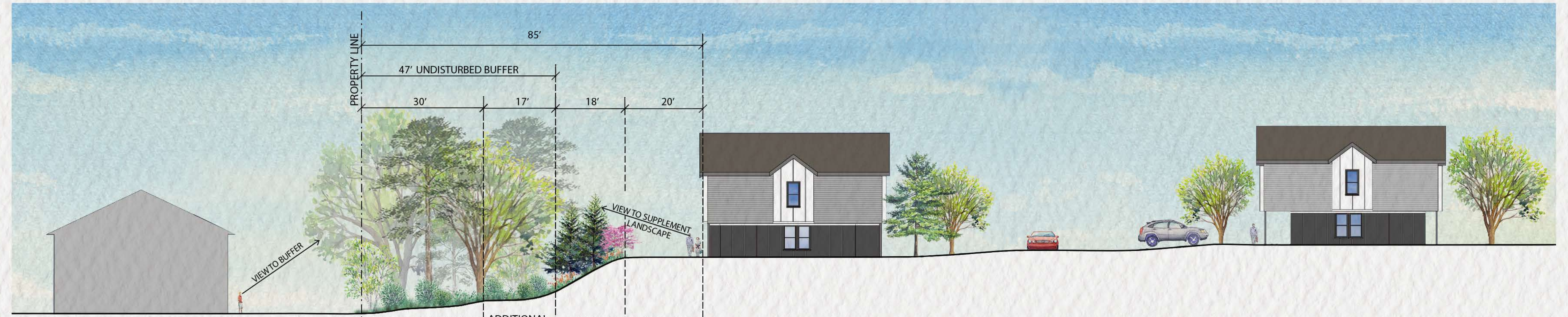
1 1-1 SECTION scale: 1"=16'-0"
